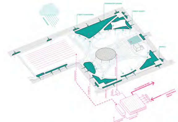
Figure 65. Stormwater management system design diagram for Northwest Resilience Park in Hoboken, NJ
