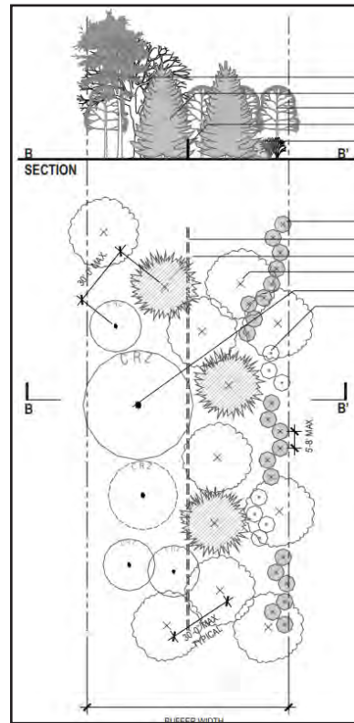
Figure 32. Buffer illustration. Source: Township of Cary, NC Community Appearance Manual
