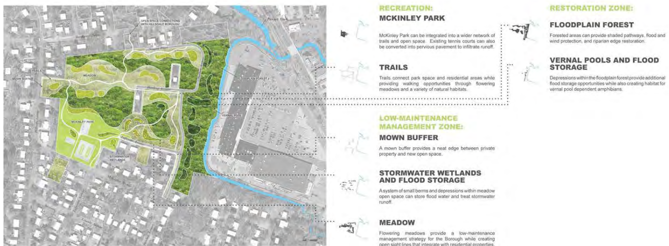
Figure 61. Resilient park designed to reduce harm from flooding. Credit: Rutgers Cooperative Extension, obtained from NJDEP's publication, Creating Flood-Resilient Landscapes.
