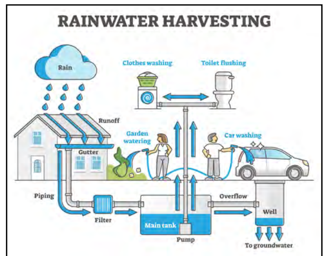
Figure 46. Diagram on the mechanics of rainwater harvesting; Adobe Stock
