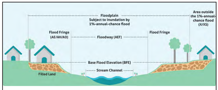
Figure 16. Riverine Flood Plain Illustration, obtained from Honolulu Planning Department.
